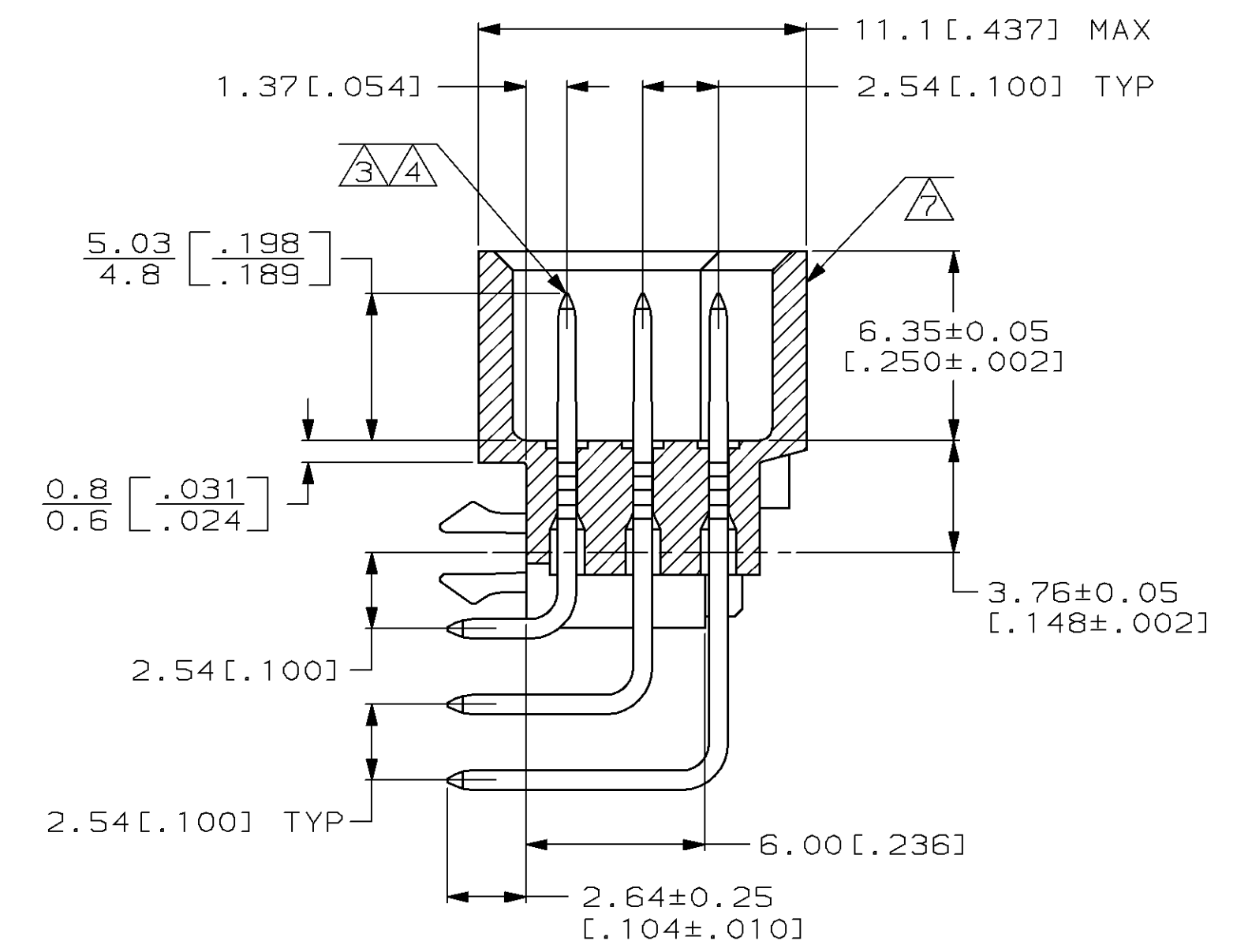
SECTION X-X
